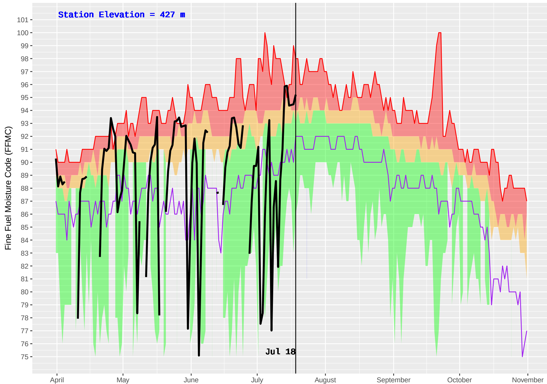
PENTICTON RS (328) : Historical (1970–2016) and Current (2018) Daily Fine Fuel Moisture Code (FFMC)
